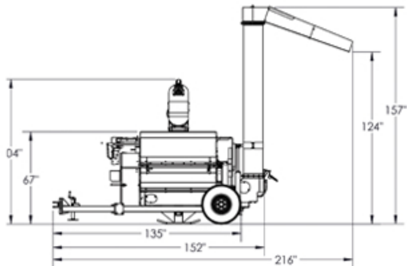
ATG6020 STANDARD INTAKE
