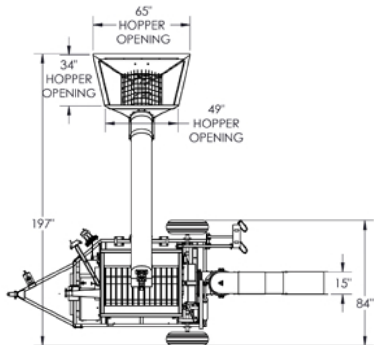
ATG6020 STANDARD INTAKE
