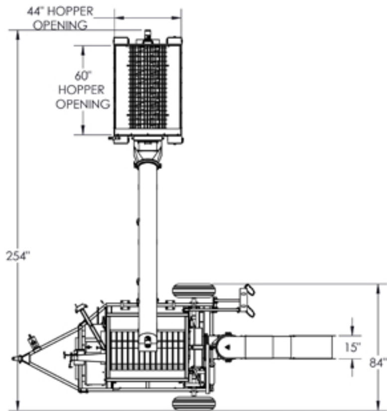
ATG6020 SWING UNDER INTAKE
